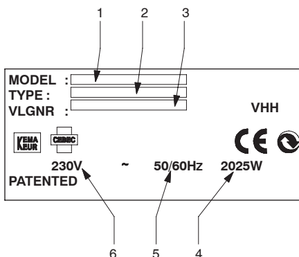
Fig. 1 Identification plate
