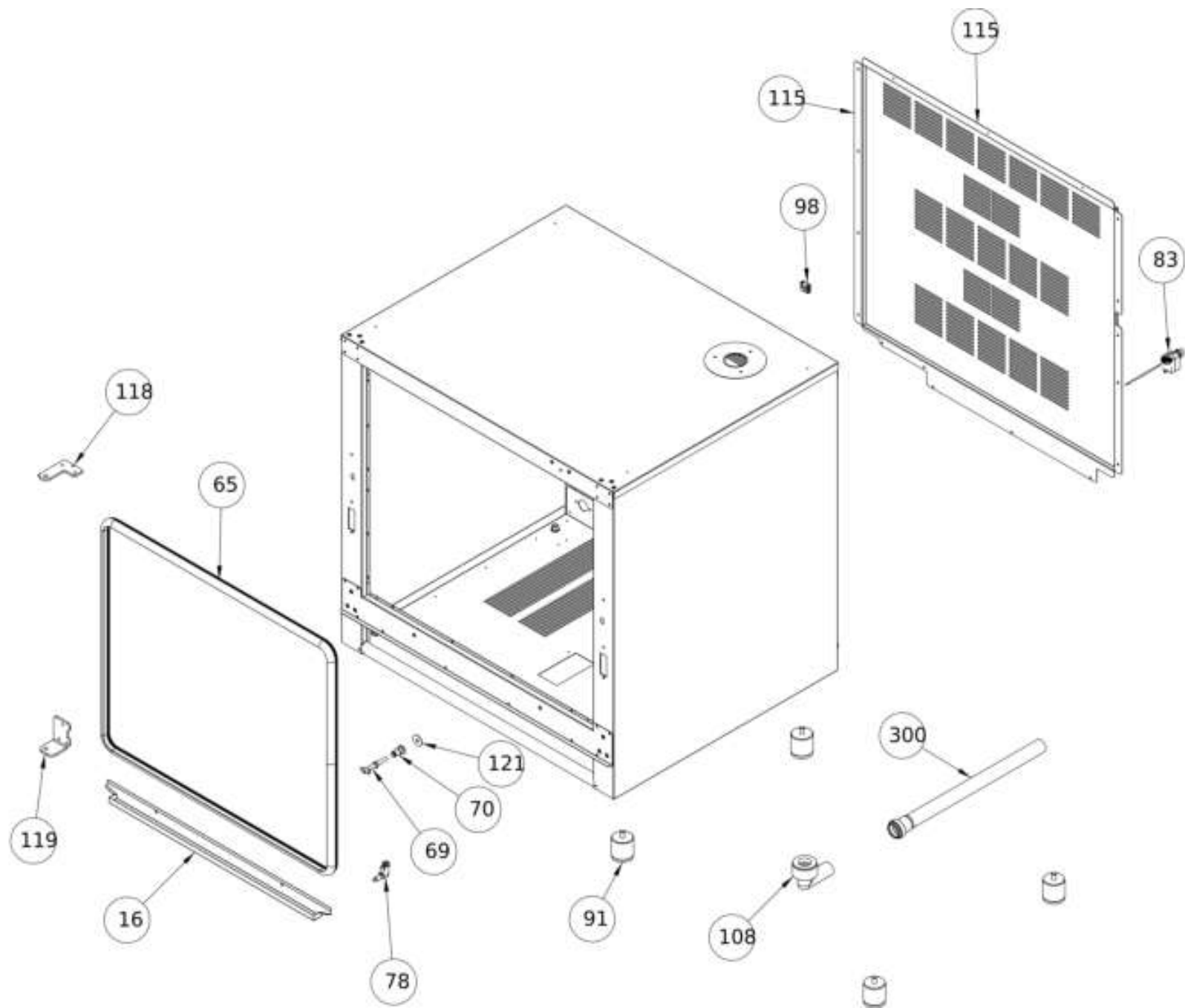
Oven body
