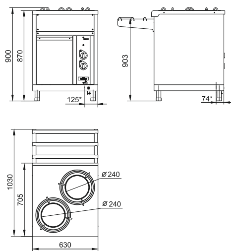
ПТЭ-70KM-80
