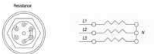
Electrical feeding variance
