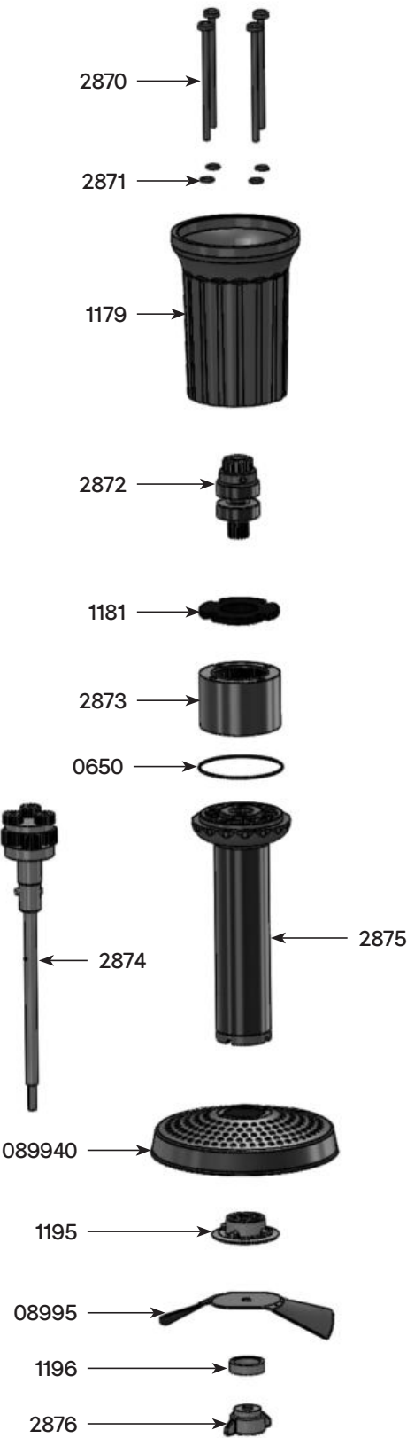
Potato ricer assembling
