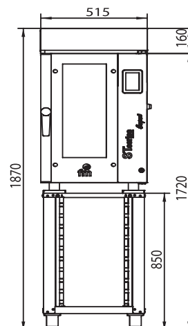
CAMPANA ST COMPACT ST-C1011 V5 SOPORTE ST-C850
