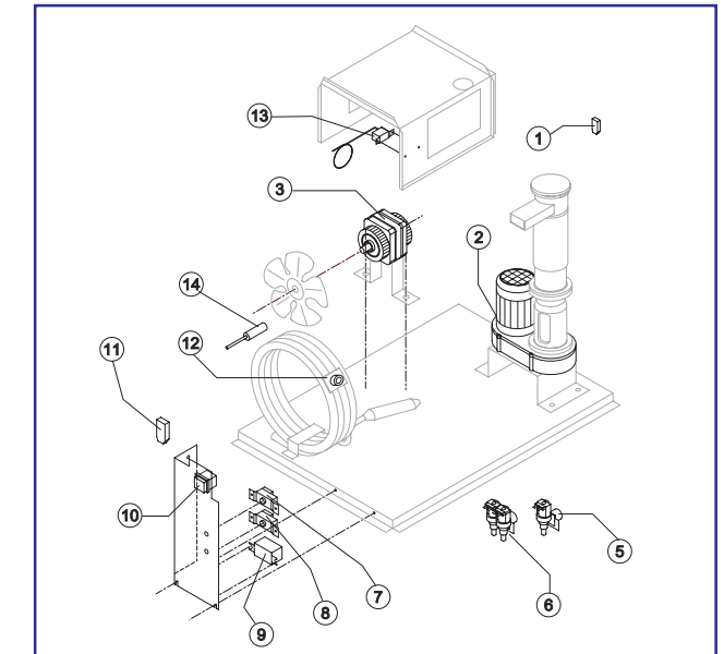
ELECTRIC PARTS
