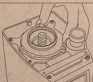
⑰ Put the upper burr holder back
