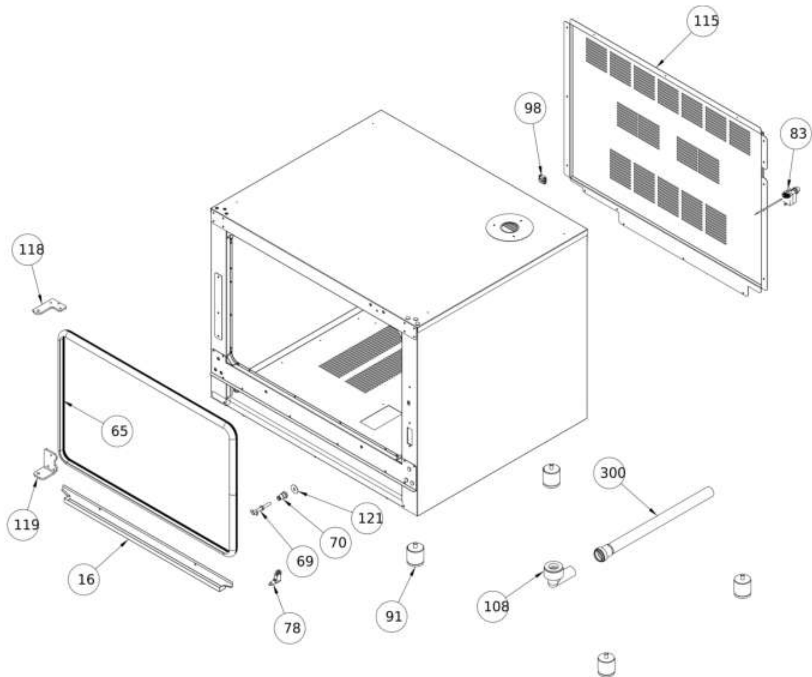
Oven body
