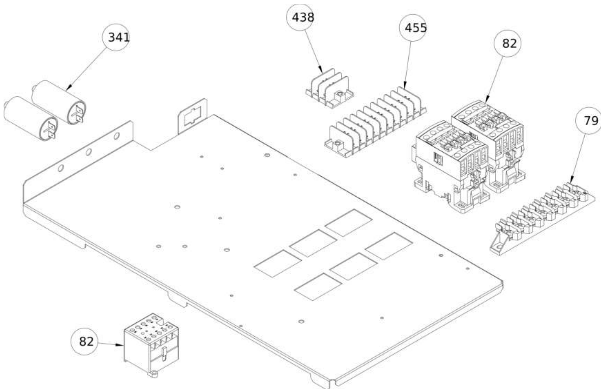
Electrical box
