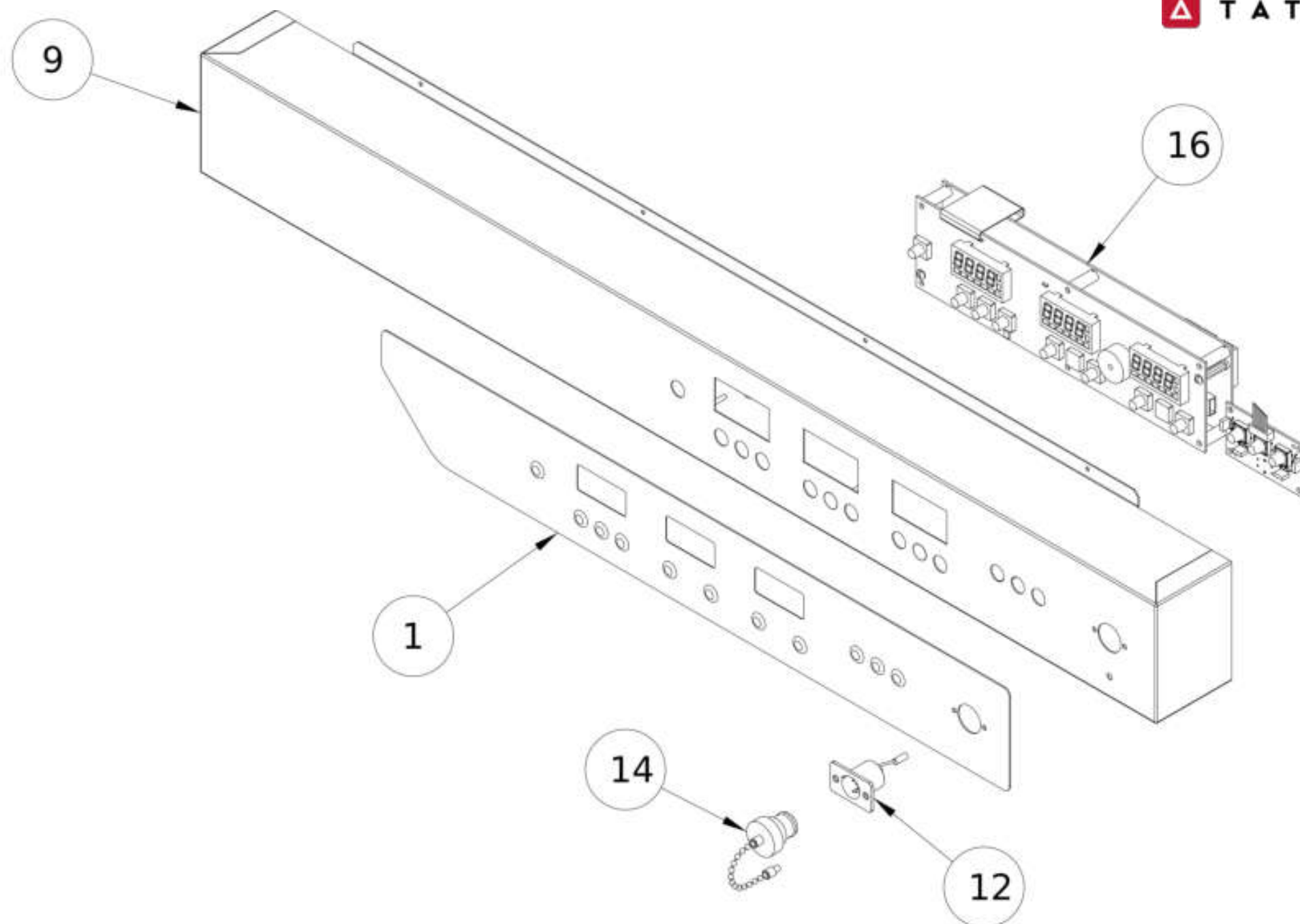
Frontal panel
