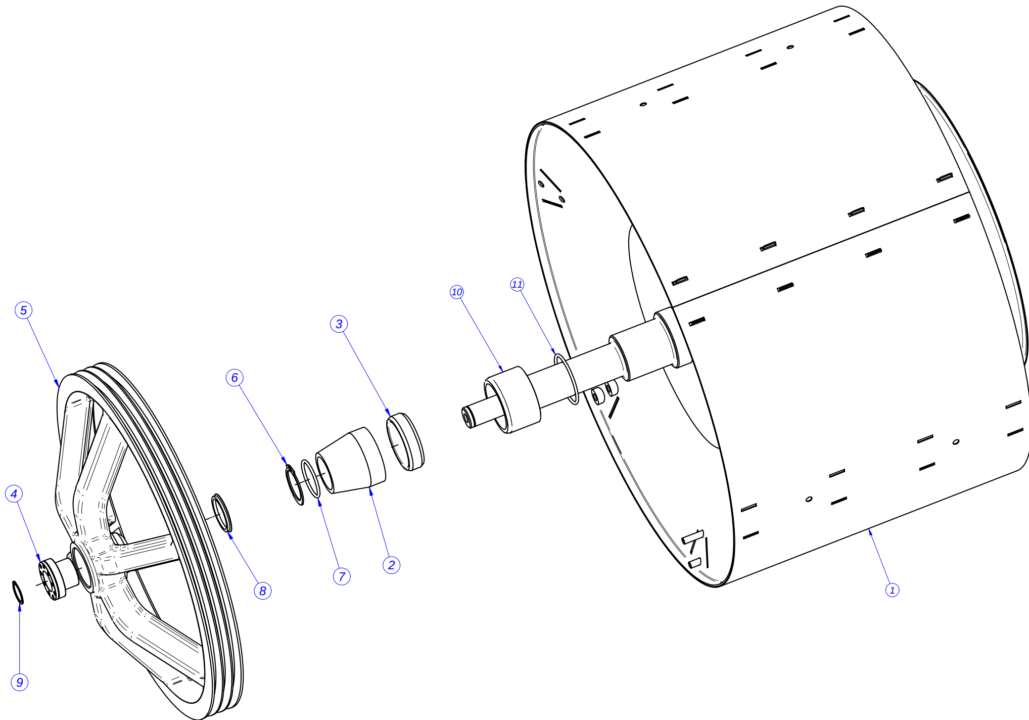
TAMBOR LA-40 / DRUM LA-40
