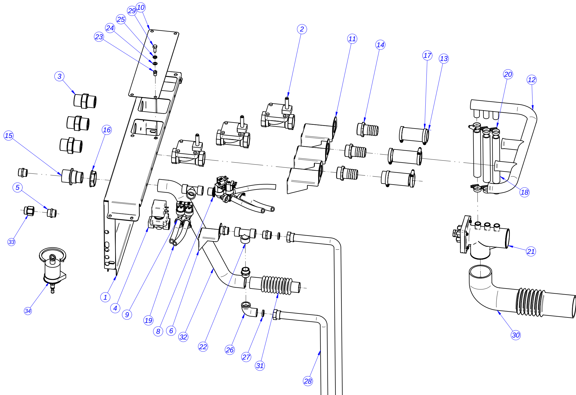
SOPORTE ELECTROVALVULAS SOLENOID VALVE SUPPORT
