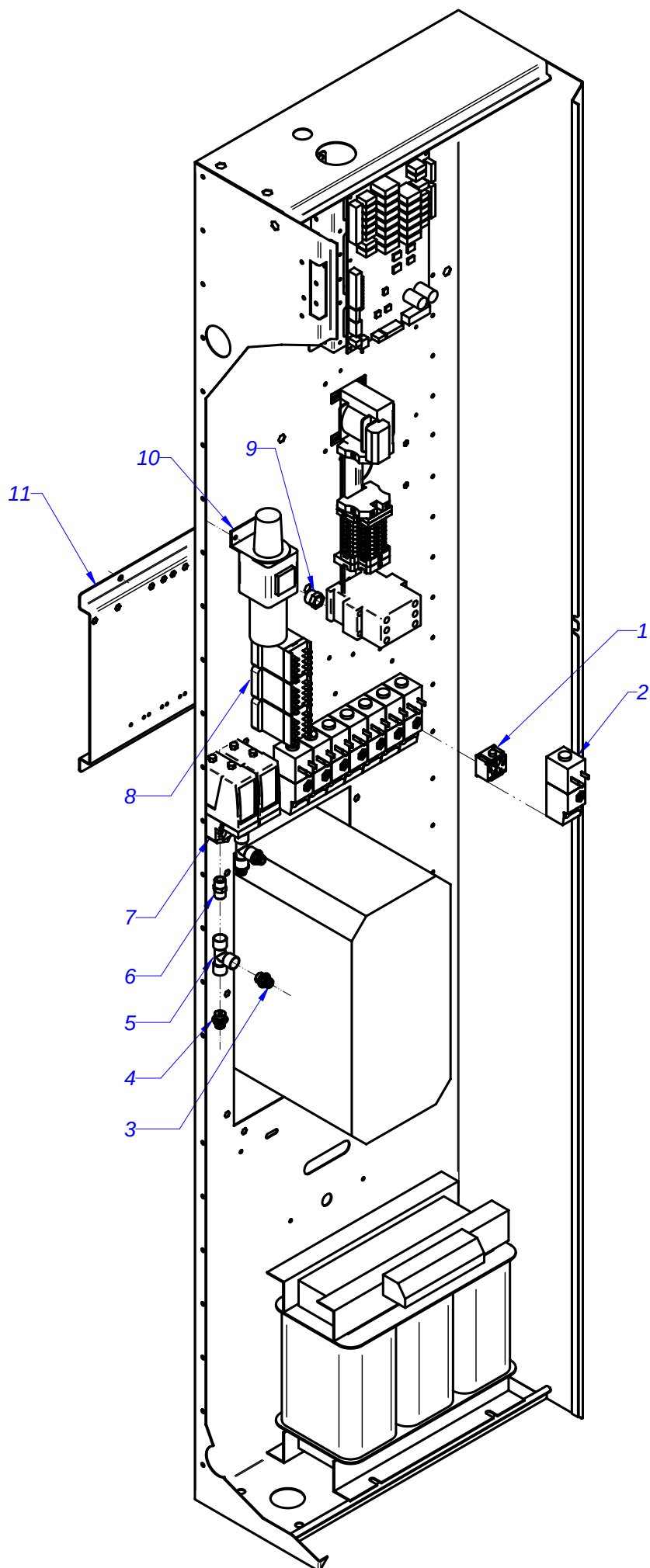
KIT BASCULACION / TILTING KIT CUADRO ELECTRICO / ELECTRIC PANEL
