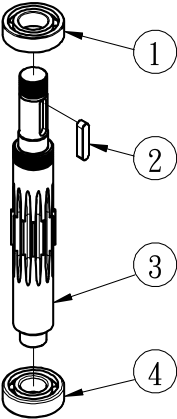
Drive Shaft Assembly
