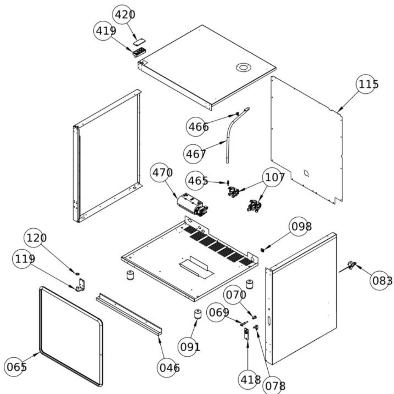
Oven body
