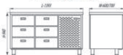
CWC-6,0-1400 / CWH-6,0-1400
