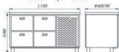
CWC-4,0-1400 / CWH-4,0-1400
