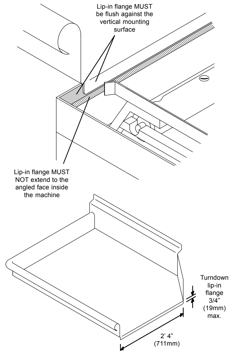
Figure 3-15: Tabling attachment
