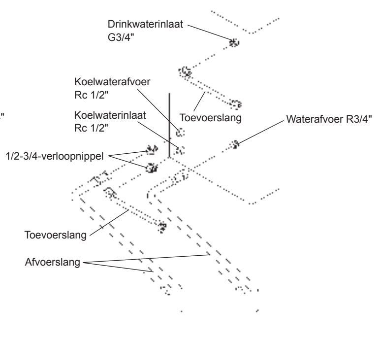
Watergekoeld model [b] (IM-45WNE/65WNE)
