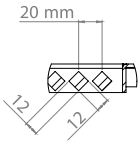
Square Rod Grate 040.04.99.005
