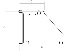
Düz Cam Flat Glass
