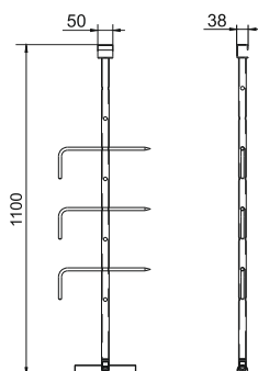
СГТ-20
