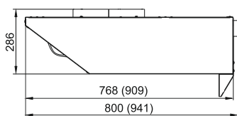
СГТ-20
