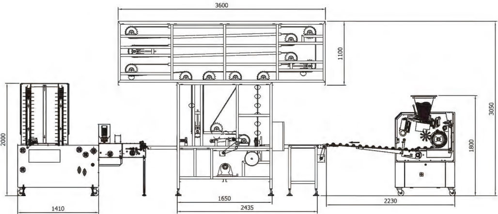
ZP-64(Platnoon machine)
